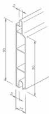
PVC hollow section profile 8367
