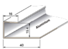
8236 Ending profile, Aluminium
