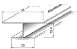
8235 T-connector profile, Aluminium
