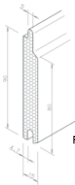
PVC profile 8081
